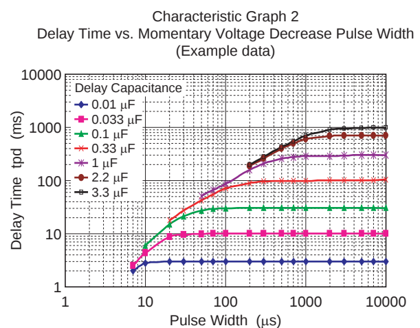
Figure 10 Characteristic Graph
